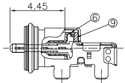
PARTIAL CROSS-SECTION A (1:1)
