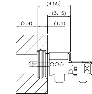
CASE INTEGRATION CONDITON(REF.)
